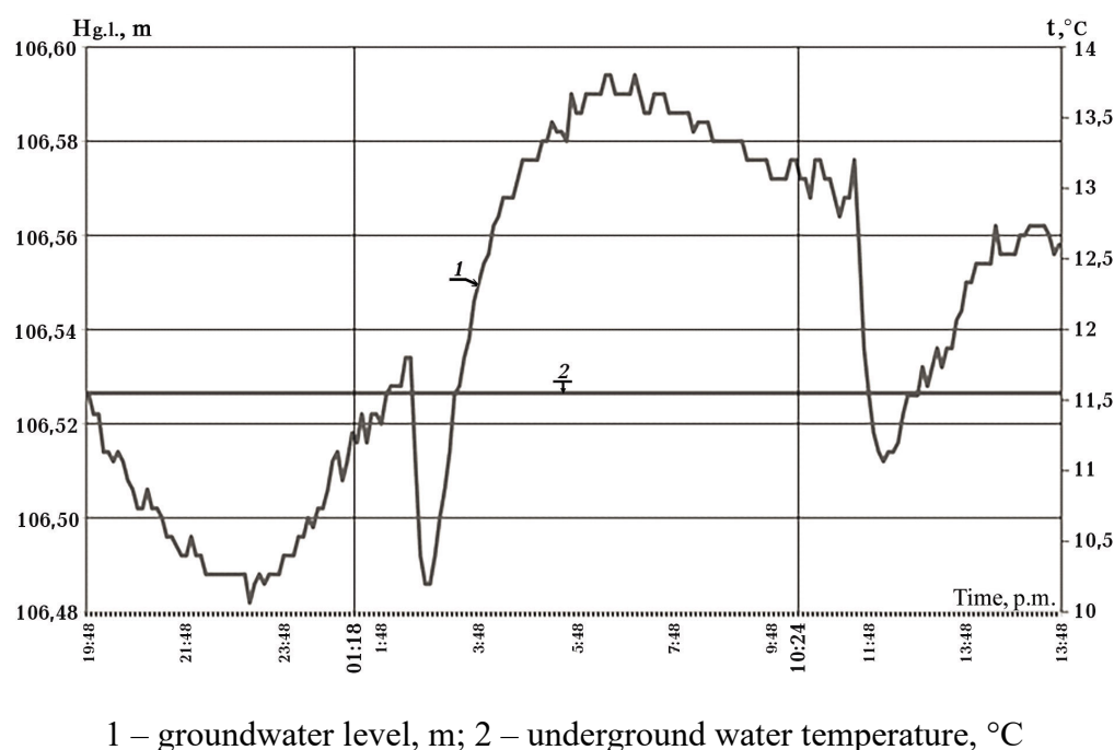
Figure 3 – Graph of groundwater level fluctuations during earthquakes in Turkey on February 6, 2023 (discrete 6 min)
